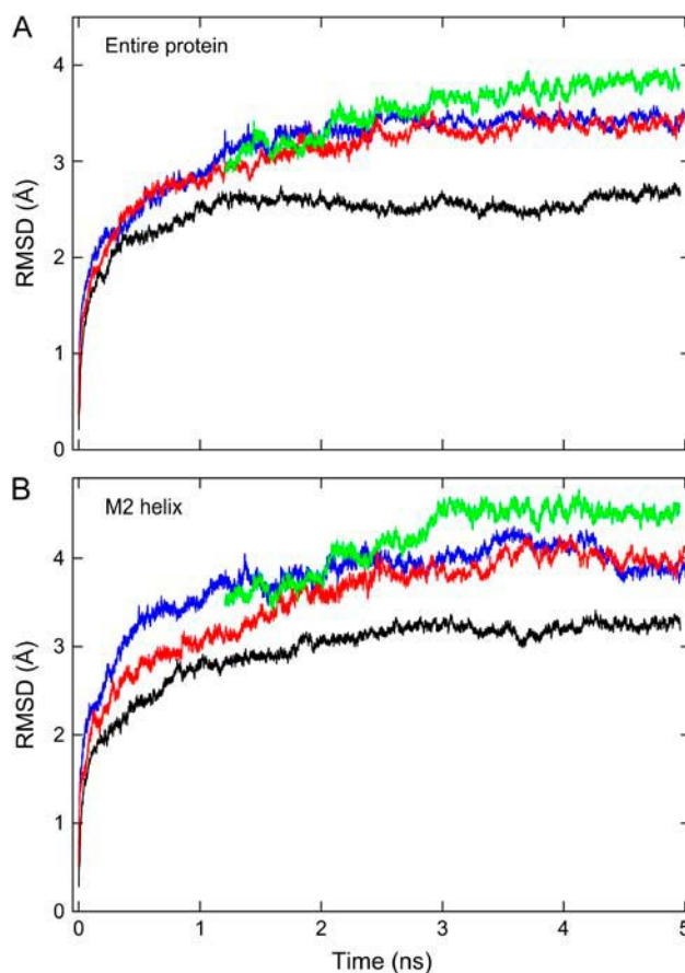
FIGURE 3 RMSD of backbone carbon atoms during MD simulations. Calculations are made for the entire protein ( A ) and M2 helix ( B ) during the simulations of the imaged ( blue ), putative open ( red ), pinned open ( black ), and V255T mutant ( green ) structures respectively.
